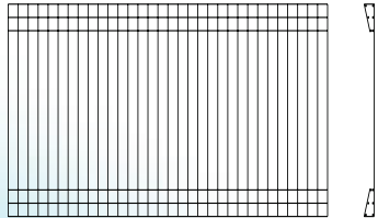
Anchor Motorway Panel 1200 High x 2400 Long
